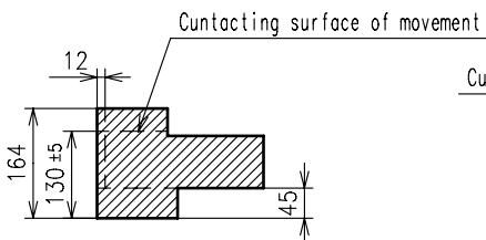
F-F' section
