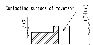
0-9H section
