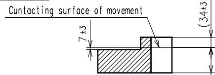
0-9H section
