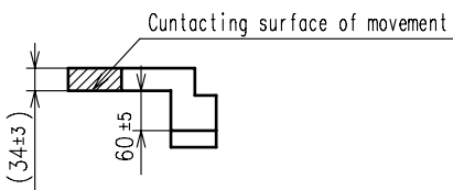
B-B' section
