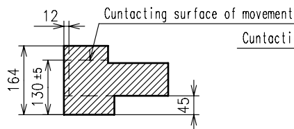
F-F' section
