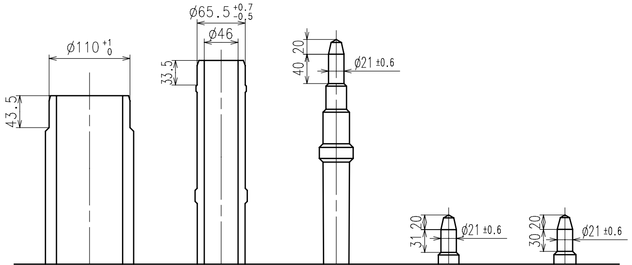
Hour wheel Center wheel 1/5 sec. chronograph wheel Small sec. wheel / Minute chronograph wheel 24 Hour wheel
