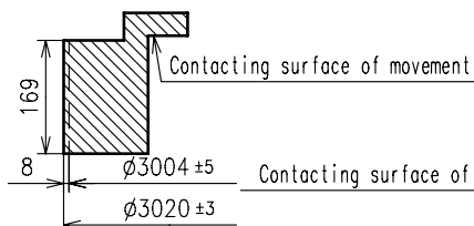
C-C' section
